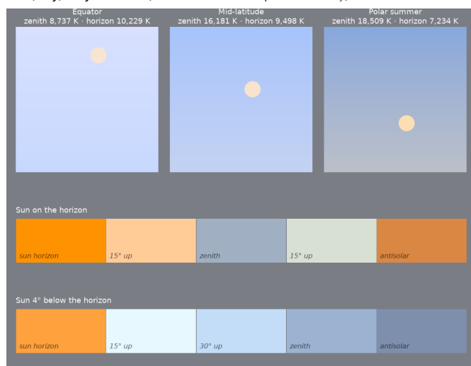
Figure 12: Snowball Earth, ~700 Ma. Top: noon sky dome at the equator, mid-latitude and polar summer, zenith at top, horizon at bottom, Sun's disk in its own color. Below: sky from the solar horizon to the antisolar horizon with the Sun on the horizon and 4° below it.
