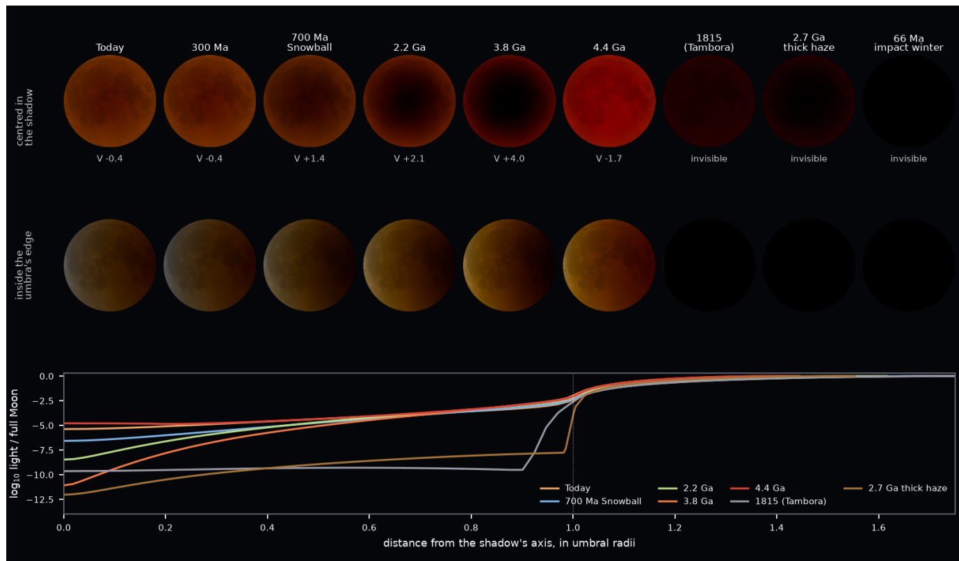
Figure 23: The Moon in the Earth's shadow at nine epochs, on today's lunar surface. Top: centered in the shadow, with its V magnitude, each drawn as the page draws it, for an eye adapted to that Moon's brightest part. Middle: just inside the umbra, its limb at 0.95 of the umbral radius, all at one exposure so their light compares: today's ozone leaves a cool gray-blue edge, the ozone-free Archean and Hadean edges are orange, and under the Tambora veil, the thick haze and the K–Pg soot the umbra is dark to its edge. Bottom: the light across the shadow, against the full Moon, with distance in units of each epoch's umbral radii.
