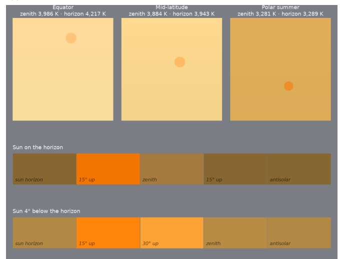
Figure 10: Neoproterozoic, ~2.7 Ga (very thick haze). Top: noon sky dome at the equator, mid-latitude and polar summer, zenith at top, horizon at bottom, Sun's disk in its own color. Below: sky from the solar horizon to the antisolar horizon with the Sun on the horizon and 4° below it.
