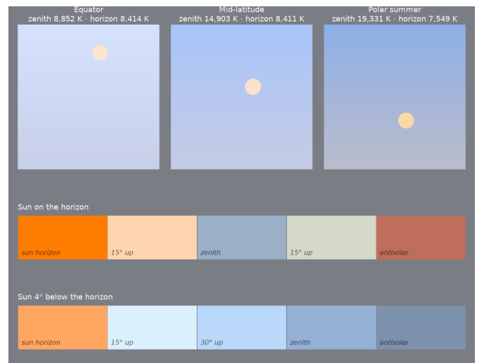
Figure 22: Year 2100. Top: noon sky dome at the equator, mid-latitude and polar summer, zenith at top, horizon at bottom, Sun's disk in its own color. Below: sky from the solar horizon to the antisolar horizon with the Sun on the horizon and 4° below it.
