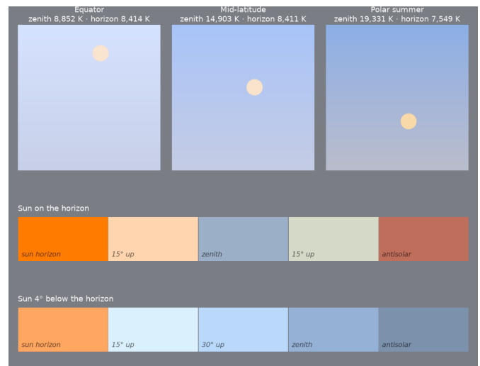
Figure 17: Geminga supernova, ~342 ka. Top: noon sky dome at the equator, mid-latitude and polar summer, zenith at top, horizon at bottom, Sun's disk in its own color. Below: sky from the solar horizon to the antisolar horizon with the Sun on the horizon and 4° below it.
