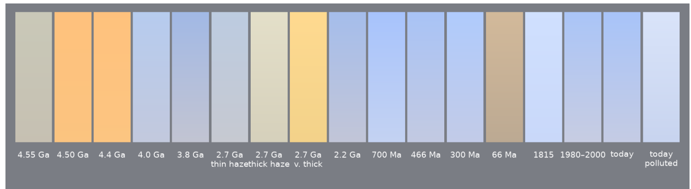
Figure 1. Mid-latitude noon sky at seventeen epochs, zenith (top) to horizon (bottom), oldest at left. Brightness shown relative to today's clean sky.
