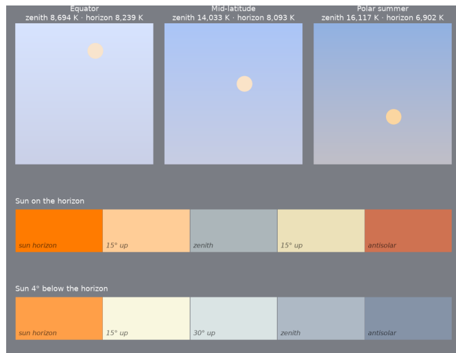
Figure 19: Ozone-hole spring. Top: noon sky dome at the equator, mid-latitude and polar summer, zenith at top, horizon at bottom, Sun's disk in its own color. Below: sky from the solar horizon to the antisolar horizon with the Sun on the horizon and 4° below it.
