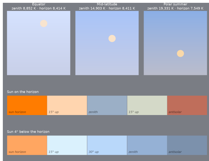
Figure 20: Modern, clean air. Top: noon sky dome at the equator, mid-latitude and polar summer, zenith at top, horizon at bottom, Sun's disk in its own color. Below: sky from the solar horizon to the antisolar horizon with the Sun on the horizon and 4° below it.
