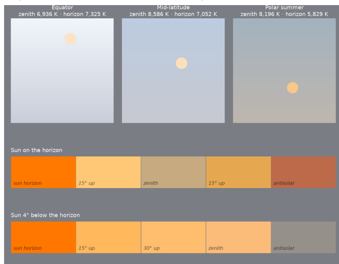
Figure 8: Neoproterozoic, ~2.7 Ga (thin haze). Top: noon sky dome at the equator, mid-latitude and polar summer, zenith at top, horizon at bottom, Sun's disk in its own color. Below: sky from the solar horizon to the antisolar horizon with the Sun on the horizon and 4° below it.
