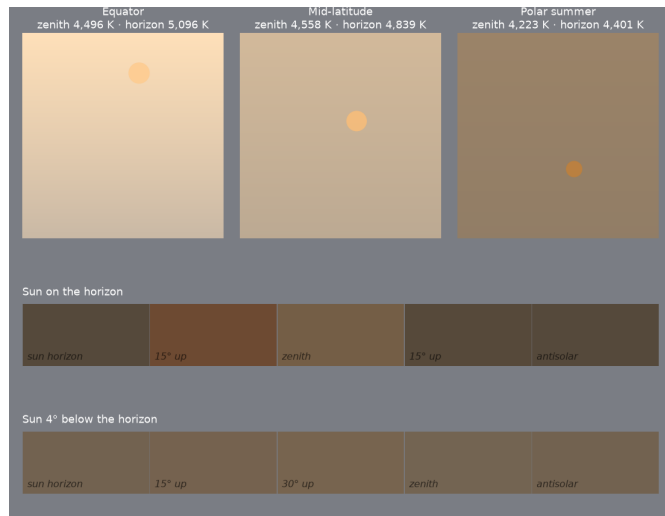
Figure 15: K-Pg impact winter, 66 Ma. Top: noon sky dome at the equator, mid-latitude and polar summer, zenith at top, horizon at bottom, Sun's disk in its own color. Below: sky from the solar horizon to the antisolar horizon with the Sun on the horizon and 4° below it.
