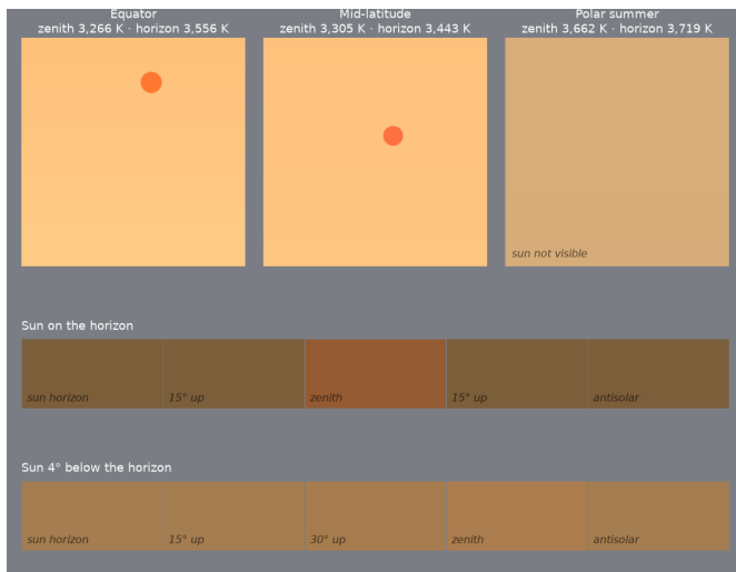
Figure 5: Early Hadean, \sim 4.4 Ga. Top: noon sky dome at the equator, mid-latitude and polar summer, zenith at top, horizon at bottom, Sun's disk in its own color. Below: sky from the solar horizon to the antisolar horizon with the Sun on the horizon and 4^\circ below it.
