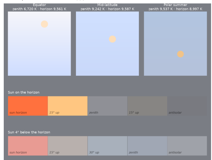
Figure 18: Volcanic year (Tambora 1815 / Toba-lite). Top: noon sky dome at the equator, mid-latitude and polar summer, zenith at top, horizon at bottom, Sun's disk in its own color. Below: sky from the solar horizon to the antisolar horizon with the Sun on the horizon and 4° below it.
