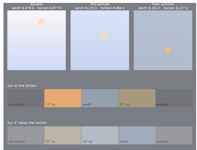
Figure 21: Modern, polluted megacity. Top: noon sky dome at the equator, mid-latitude and polar summer, zenith at top, horizon at bottom, Sun's disk in its own color. Below: sky from the solar horizon to the antisolar horizon with the Sun on the horizon and 4° below it.
