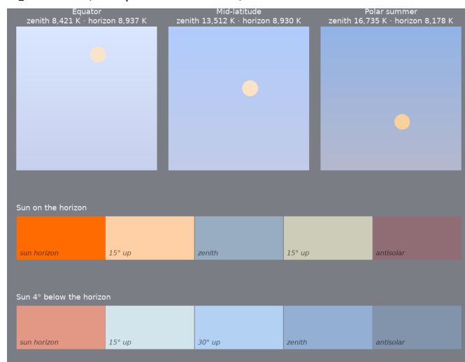
Figure 14: Carboniferous, ~300 Ma. Top: noon sky dome at the equator, mid-latitude and polar summer, zenith at top, horizon at bottom, Sun's disk in its own color. Below: sky from the solar horizon to the antisolar horizon with the Sun on the horizon and 4° below it.
