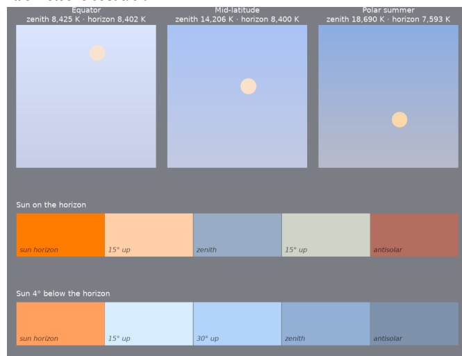
Figure 13: Ordovician meteor storm, ~466 Ma. Top: noon sky dome at the equator, mid-latitude and polar summer, zenith at top, horizon at bottom, Sun's disk in its own color. Below: sky from the solar horizon to the antisolar horizon with the Sun on the horizon and 4° below it.
