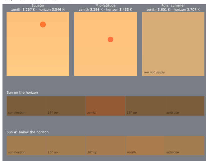
Figure 4: Earliest Hadean, ~4.50 Ga. Top: noon sky dome at the equator, mid-latitude and polar summer, zenith at top, horizon at bottom, Sun's disk in its own color. Below: sky from the solar horizon to the antisolar horizon with the Sun on the horizon and 4° below it.
