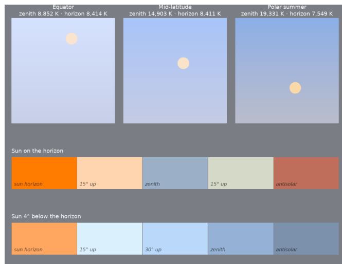
Figure 16: ζ Ophiuchi supernova, ~1.78 Ma. Top: noon sky dome at the equator, mid-latitude and polar summer, zenith at top, horizon at bottom, Sun's disk in its own color. Below: sky from the solar horizon to the antisolar horizon with the Sun on the horizon and 4° below it.
