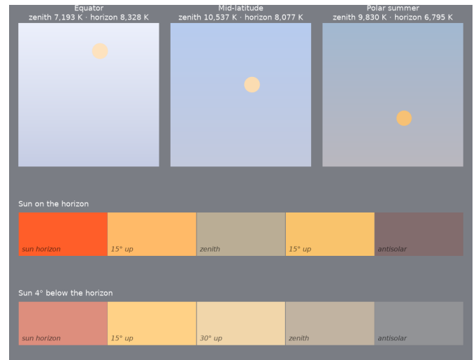
Figure 6: Late Hadean, \sim 4.0 Ga. Top: noon sky dome at the equator, mid-latitude and polar summer, zenith at top, horizon at bottom, Sun's disk in its own color. Below: sky from the solar horizon to the antisolar horizon with the Sun on the horizon and 4^\circ below it.
