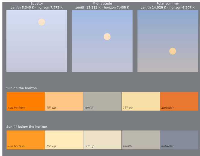
Figure 7: Early Archean, ~3.8 Ga. Top: noon sky dome at the equator, mid-latitude and polar summer, zenith at top, horizon at bottom, Sun's disk in its own color. Below: sky from the solar horizon to the antisolar horizon with the Sun on the horizon and 4° below it.
