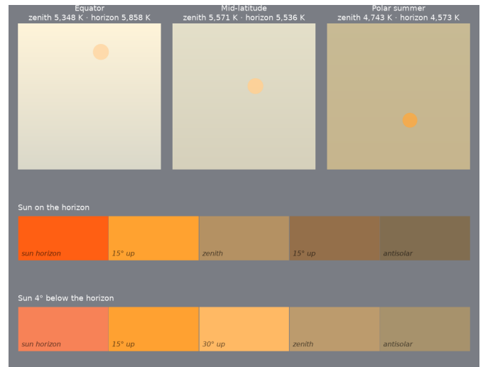
Figure 9: Neoproterozoic, ~2.7 Ga (thick haze). Top: noon sky dome at the equator, mid-latitude and polar summer, zenith at top, horizon at bottom, Sun's disk in its own color. Below: sky from the solar horizon to the antisolar horizon with the Sun on the horizon and 4° below it.
