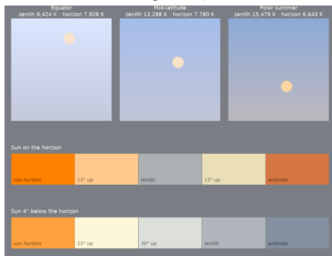
Figure 11: Paleoproterozoic, ~2.2 Ga. Top: noon sky dome at the equator, mid-latitude and polar summer, zenith at top, horizon at bottom, Sun's disk in its own color. Below: sky from the solar horizon to the antisolar horizon with the Sun on the horizon and 4° below it.
