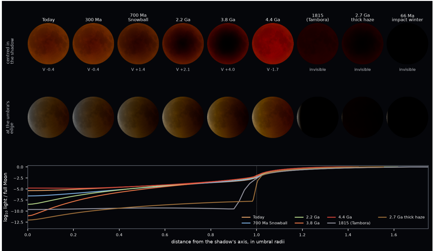
Figure 21: The Moon in the Earth's shadow at nine epochs. Top: centered in the shadow, with its V magnitude. Middle: just inside the umbra's edge, where today's ozone leaves a cool gray-blue edge and the ozone-free Archean and Hadean edges are orange. Each Moon is drawn as the page draws it, for an eye adapted to its brightest part, on today's lunar surface. Bottom: the light across the shadow, against the full Moon, with distance in units of each epoch's umbral radius.
