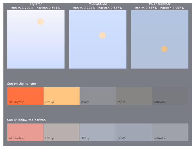
Figure 16: Volcanic year (Tambora 1815 / Toba-lite). Top: noon sky dome at the equator, mid-latitude and polar summer, zenith at top, horizon at bottom, Sun's disk in its own color. Below: sky from the solar horizon to the antisolar horizon with the Sun on the horizon and 4^\circ below it.
