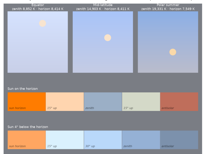
Figure 14: ζ Ophiuchi supernova, ~1.78 Ma. Top: noon sky dome at the equator, mid-latitude and polar summer, zenith at top, horizon at bottom, Sun's disk in its own color. Below: sky from the solar horizon to the antisolar horizon with the Sun on the horizon and 4° below it.
