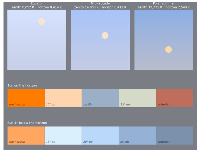
Figure 20: Year 2100. Top: noon sky dome at the equator, mid-latitude and polar summer, zenith at top, horizon at bottom, Sun's disk in its own color. Below: sky from the solar horizon to the antisolar horizon with the Sun on the horizon and 4° below it.
