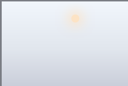
Equator zenith 6,936 K · horizon 7,325 K
