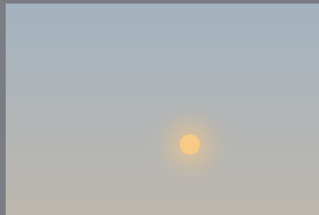
Polar summer zenith 8,196 K · horizon 5,829 K
