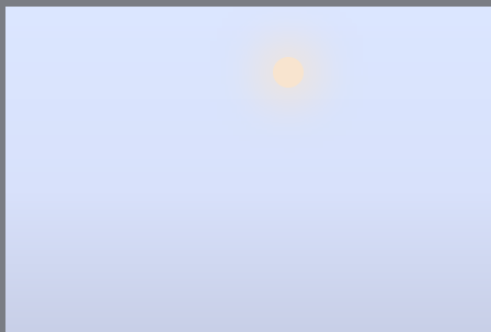
Equator zenith 8,425 K · horizon 8,402 K
