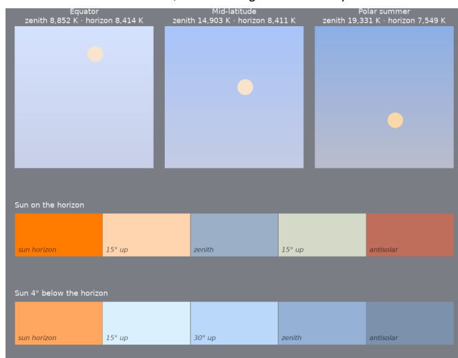
Figure 15: Geminga supernova, ~342 ka. Top: noon sky dome at the equator, mid-latitude and polar summer, zenith at top, horizon at bottom, Sun's disk in its own color. Below: sky from the solar horizon to the antisolar horizon with the Sun on the horizon and 4° below it.
