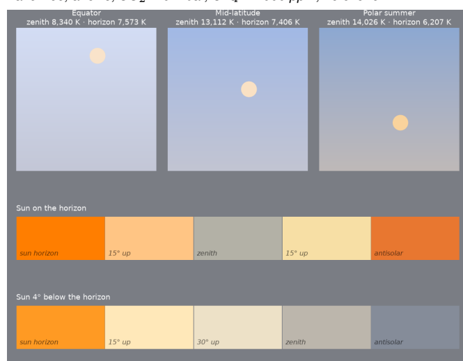
Figure 5: Early Archean, \sim 3.8 Ga. Top: noon sky dome at the equator, mid-latitude and polar summer, zenith at top, horizon at bottom, Sun's disk in its own color. Below: sky from the solar horizon to the antisolar horizon with the Sun on the horizon and 4^\circ below it.
