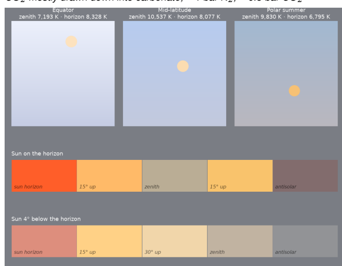
Figure 4: Late Hadean, \sim 4.0 Ga. Top: noon sky dome at the equator, mid-latitude and polar summer, zenith at top, horizon at bottom, Sun's disk in its own color. Below: sky from the solar horizon to the antisolar horizon with the Sun on the horizon and 4^\circ below it.
