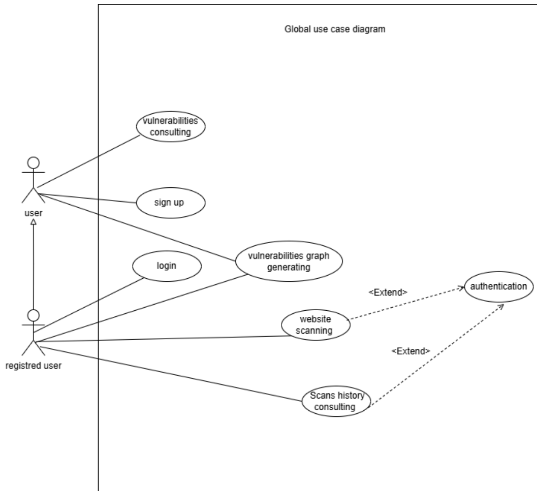
Figure 2.2: Global Use Case Diagram of CyberScope
