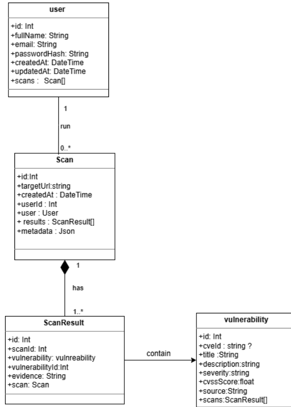
Figure 2.3: Global Class Diagram of CyberScope
