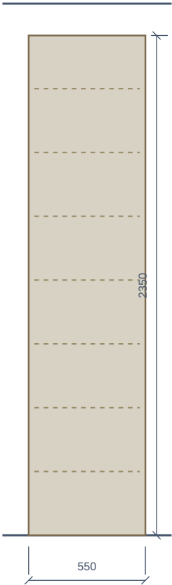
SHOE TOWER · 1:25 550×350×2350 · 10 pairs · looking south
