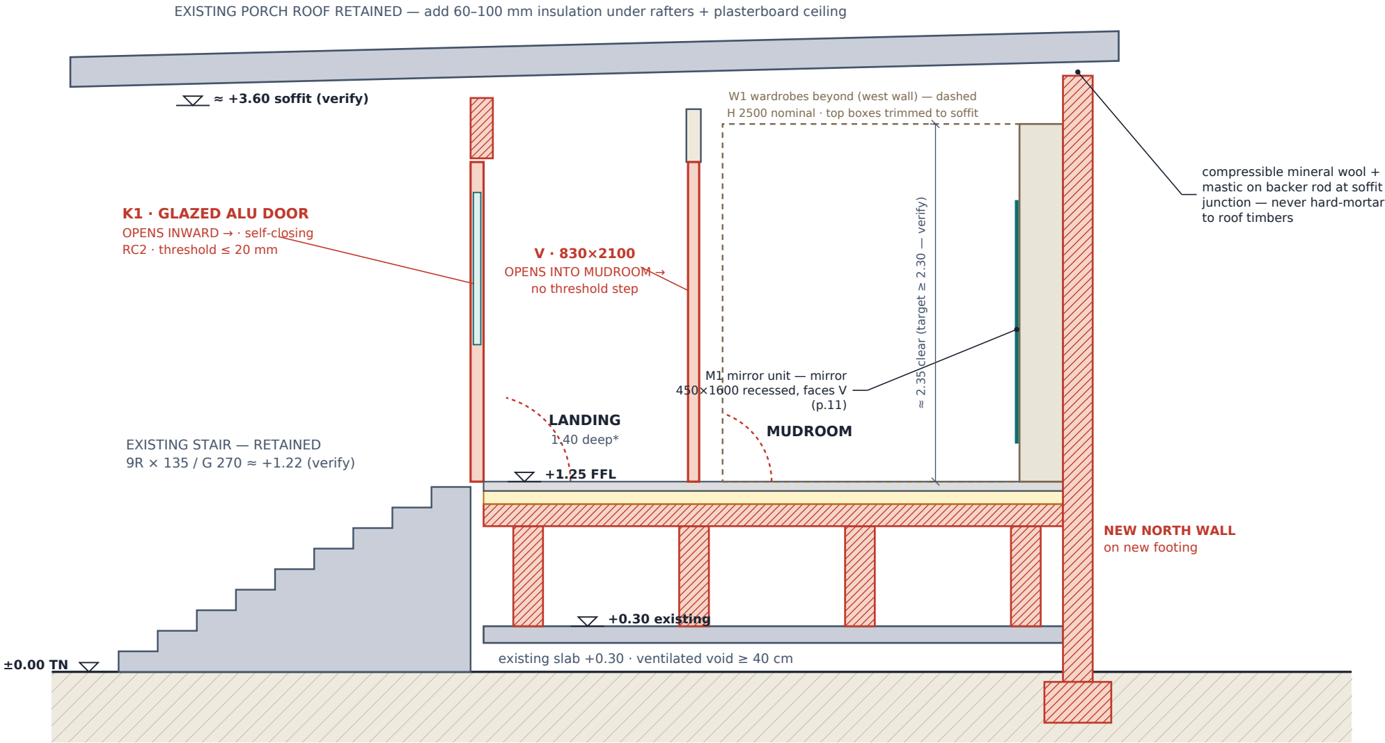
SECTION B-B · SCALE ≈ 1:35 @ A3 · developed along the entry path (up the stair, through K1, across the landing, through V, to the mirror)
