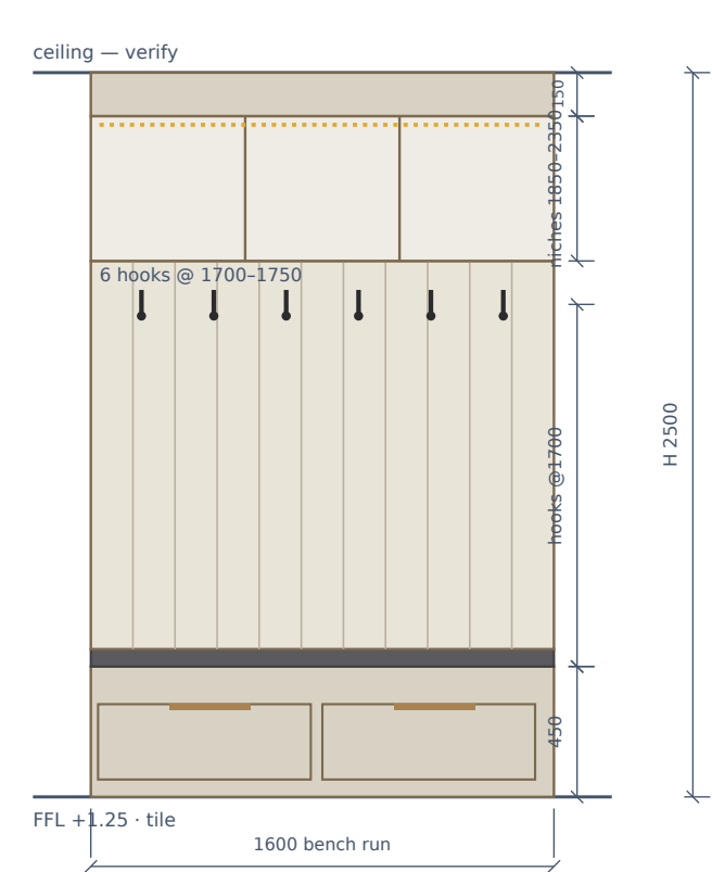
ELEVATION B1 · ≈ 1:28 @ A3 east wall — former door built solid, full wall usable
