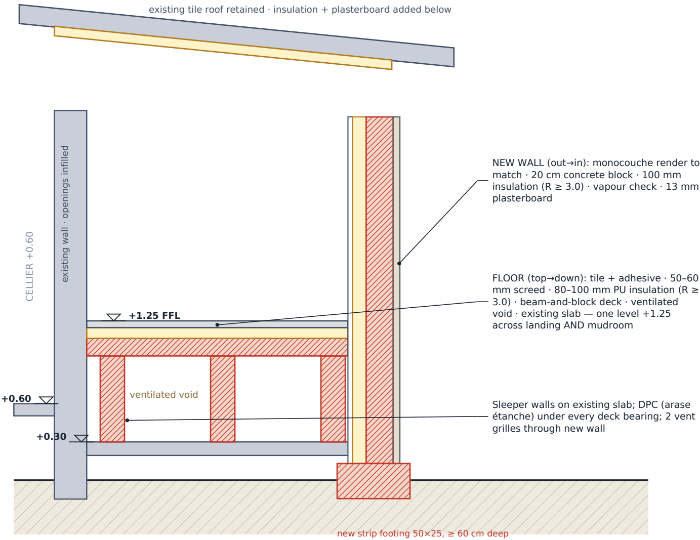
SECTION A-A · ≈ 1:25 @ A3 · looking north
