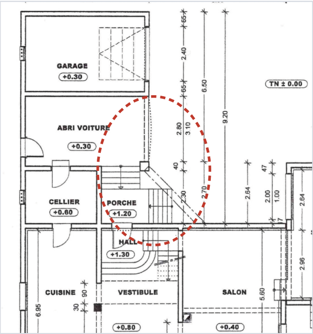
4 · RDC permit plan extract (2006) — porch zone
