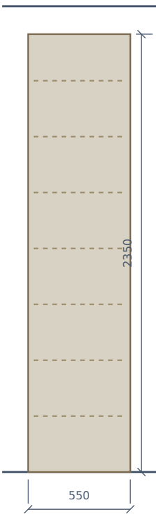
SHOE TOWER · ≈ 1:28 550×350×2350 · ≈ 10 pairs on the partition, east end (anti-tip fixing only)
