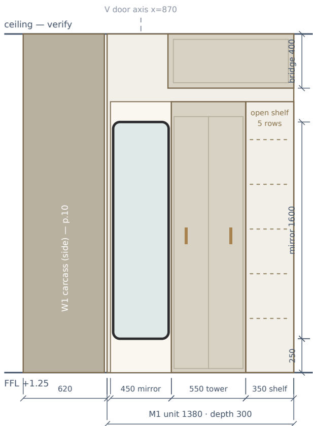
M1 — NORTH WALL · ≈ 1:28 @ A3 mirror recessed on the V-door axis — the entrant faces it; west side abuts W1
