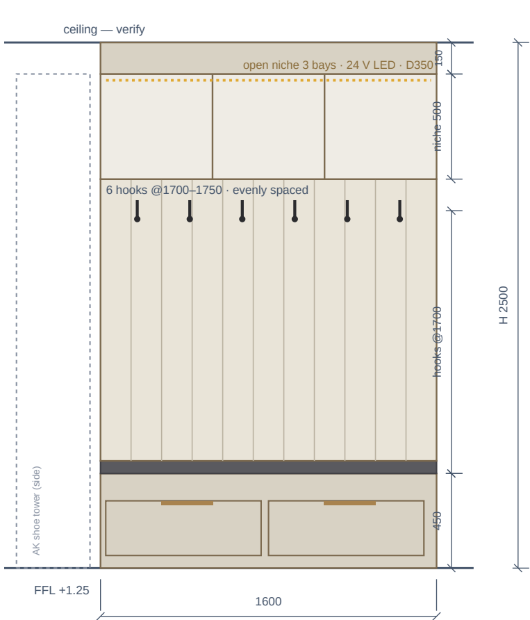
B1 ELEVATION (LOOKING EAST) · 1:25 east wall — full wall now the old door is bricked up; 2 Tandembox drawers glazing band CANCELLED (owner decision, Faz 4.2) — east wall solid; daylight via K1 glazing
