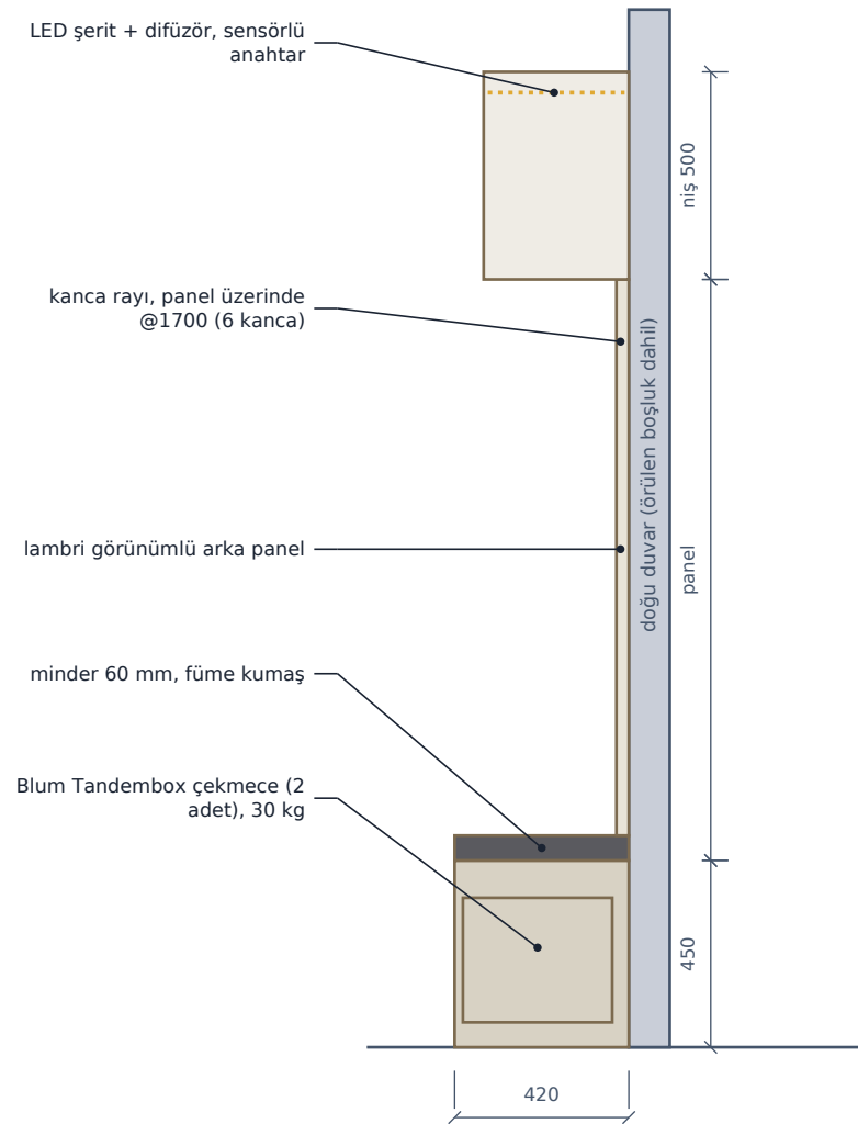
KESİT 1 — BANK DUVARI B1 · 1:20
