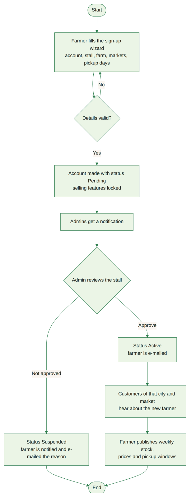
Figure 7 – Farmer registration and approval
