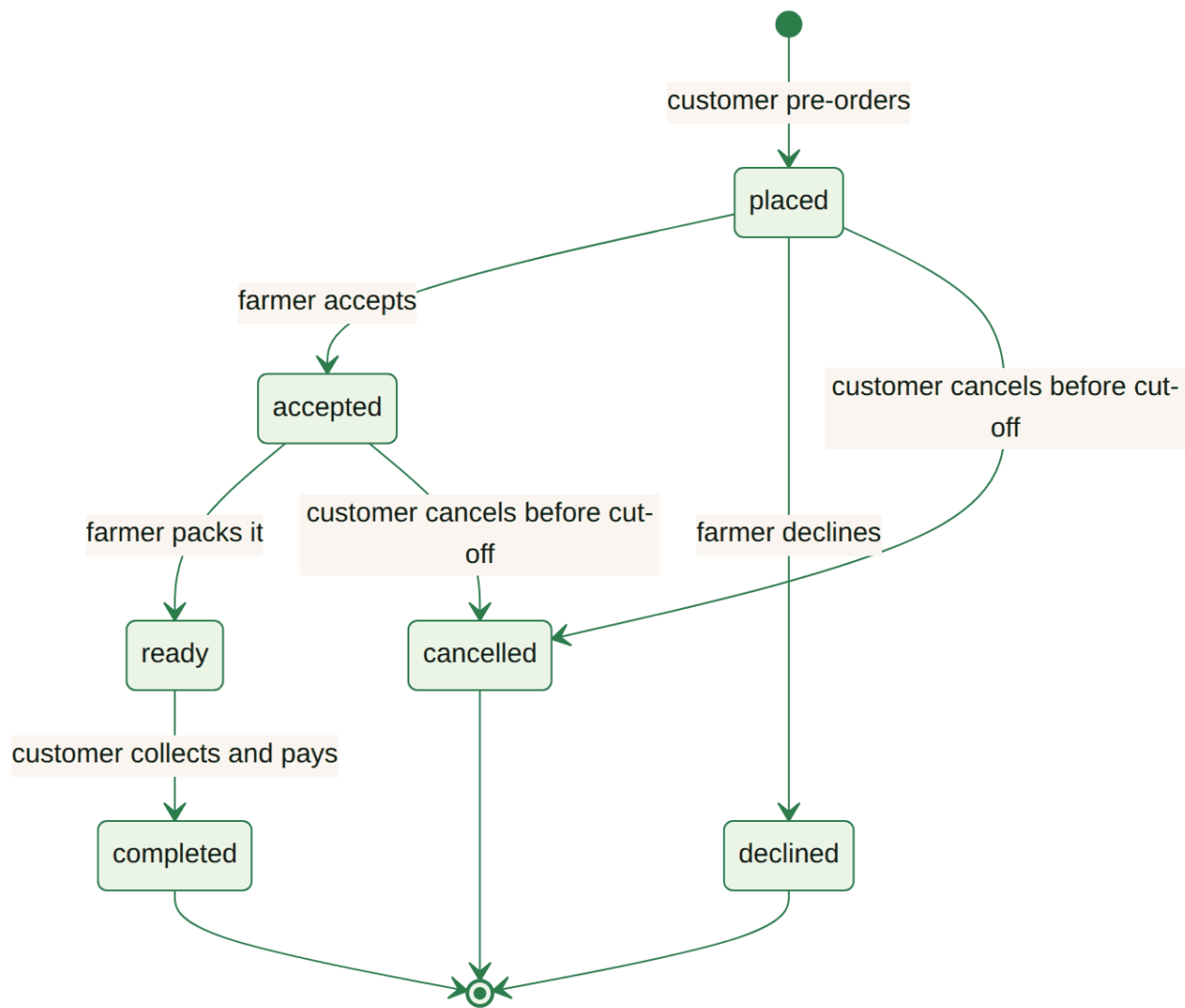
Figure 11 – Order status diagram
