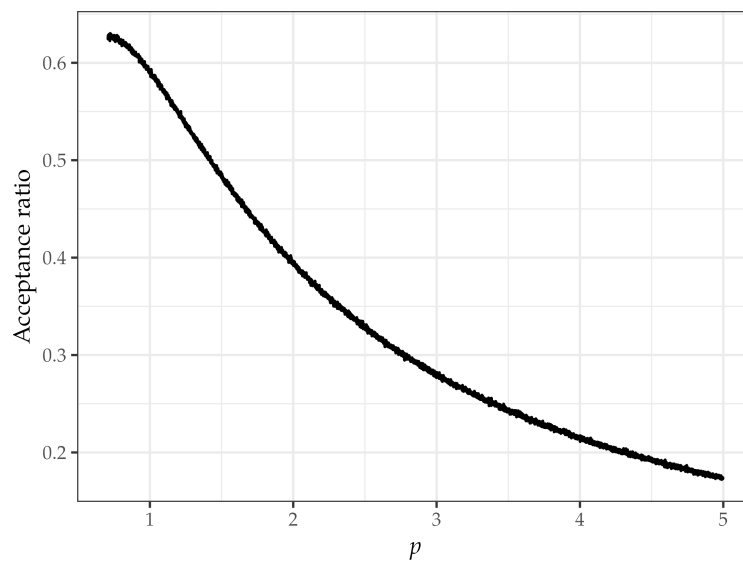
Figure 2.3.2: acceptance ratio over 100 000 samples as a function of p in Ex. 2.3.
