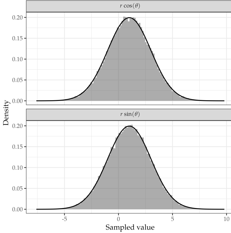
Figure 2.2.1: histograms of 100 000 samples – half in the upper panel, half in the lower one – from a N(1, 4) distribution, obtained with the Box–Muller method. The theoretical distribution is overlaid with a solid line.
