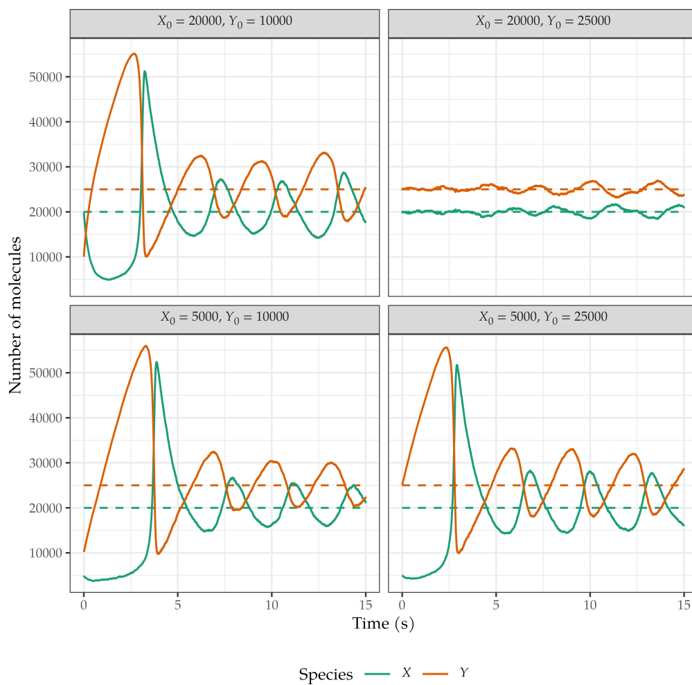
Figure 6.2.3: first set of Brusselator simulations, with a = 2 \text{ s}^{-1} , b = 5 \text{ s}^{-1} and volume \Omega = 10^4 . The initial conditions are reported above each plot and the stationary solution (a\Omega, b\Omega/a) is highlighted with dashed lines.
