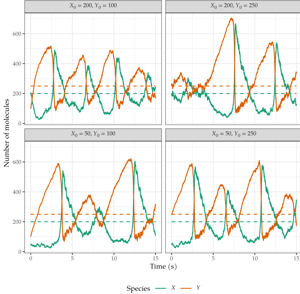
Figure 6.2.1: first set of Brusselator simulations, with a = 2 \text{ s}^{-1} , b = 5 \text{ s}^{-1} and volume \Omega = 10^2 . The initial conditions are reported above each plot and the stationary solution (a\Omega, b\Omega/a) is highlighted with dashed lines.
