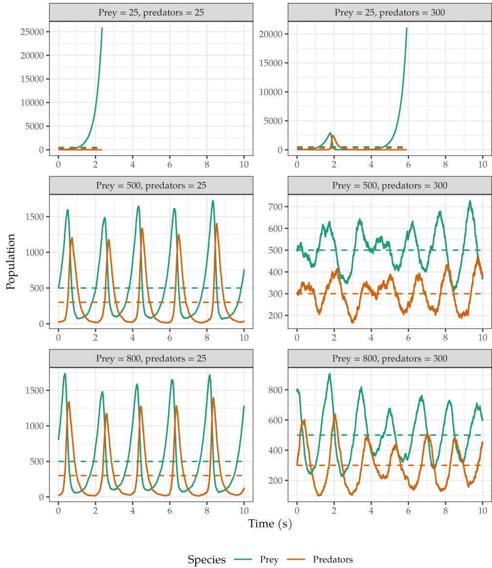
Figure 6.1.1: first set of Lotka–Volterra simulations with k_1 = 3 \text{ s}^{-1} , k_2 = 0.01 \text{ s}^{-1} and k_3 = 5 \text{ s}^{-1} . The initial conditions are reported above each plot and the stationary solution (k_3/k_2, k_1/k_2) is highlighted with dashed lines.
