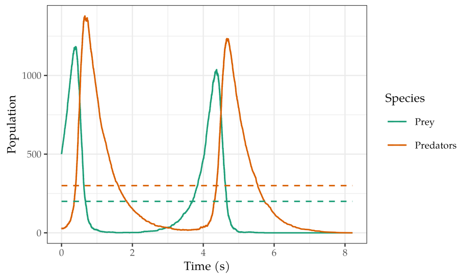
Figure 6.1.4: simulation of the Lotka–Volterra model with k_1 = 3 \text{ s}^{-1} , k_2 = 0.01 \text{ s}^{-1} and k_3 = 2 \text{ s}^{-1} .
