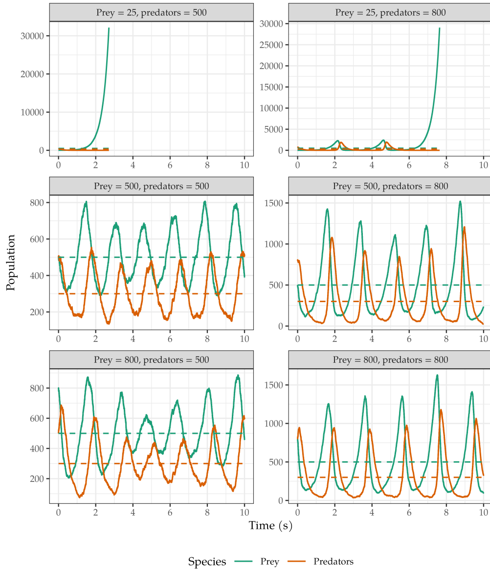
Figure 6.1.2: second set of Lotka–Volterra simulations with k_1 = 3 \text{ s}^{-1} , k_2 = 0.01 \text{ s}^{-1} and k_3 = 5 \text{ s}^{-1} . The initial conditions are reported above each plot and the stationary solution ( k_3/k_2, k_1/k_2 ) is highlighted with dashed lines.
