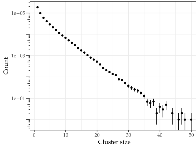
Figure 5.1.3: histogram of cluster sizes obtained from a Wolff algorithm simulation with N = 2500 spins, run at a temperature T = 2T_c over 500 000 time steps. Error bars represent Poissonian uncertainties.
