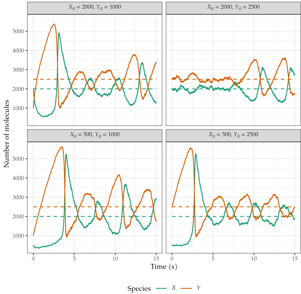
Figure 6.2.2: first set of Brusselator simulations, with a = 2 \text{ s}^{-1} , b = 5 \text{ s}^{-1} and volume \Omega = 10^3 . The initial conditions are reported above each plot and the stationary solution (a\Omega, b\Omega/a) is highlighted with dashed lines.
