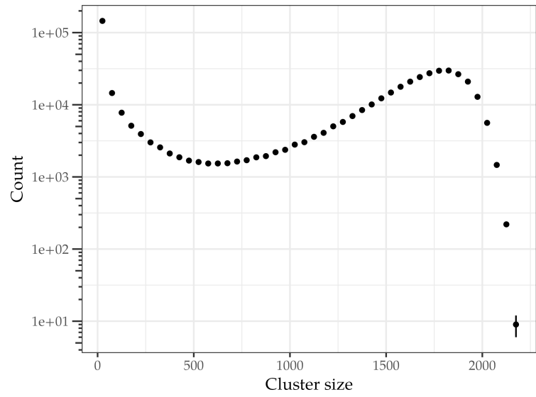
Figure 5.1.2: histogram of cluster sizes obtained from a Wolff algorithm simulation with N = 2500 spins, run at a temperature T = T_c over 500 000 time steps. Error bars represent Poissonian uncertainties.
