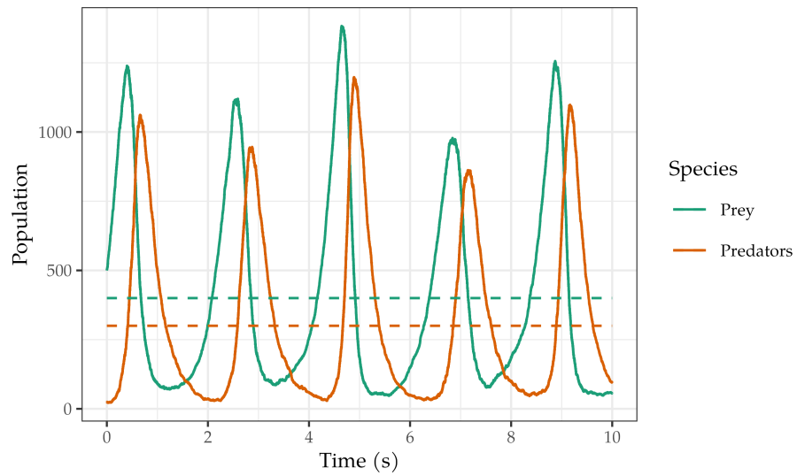
Figure 6.1.3: simulation of the Lotka–Volterra model with k_1 = 3 \text{ s}^{-1} , k_2 = 0.01 \text{ s}^{-1} and k_3 = 4 \text{ s}^{-1} .
