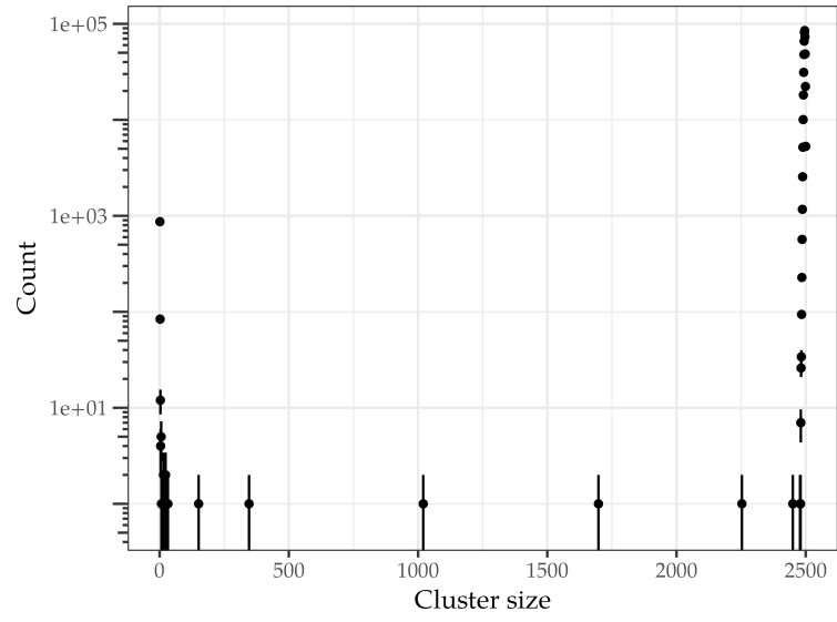
Figure 5.1.1: histogram of cluster sizes obtained from a Wolff algorithm simulation with N = 2500 spins, run at a temperature T = T_c/2 over 500 000 time steps. Error bars represent Poissonian uncertainties.
