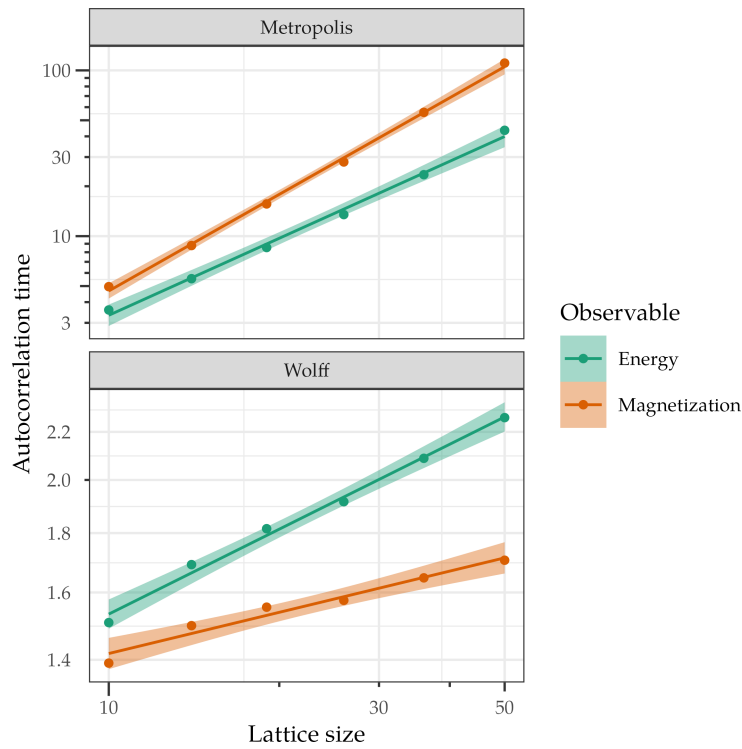
Figure 5.1.4: autocorrelation time of energy and magnetization as a function of the lattice size for the Metropolis and Wolff algorithms. Each run lasted 1 000 000 time steps. The parameters of the fitted lines are reported in table 5.1.1.
