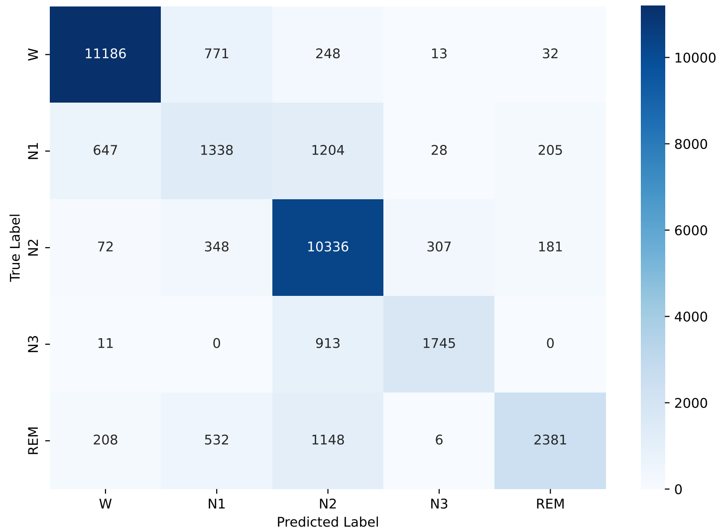
Confusion Matrix - FusionBiLSTM
