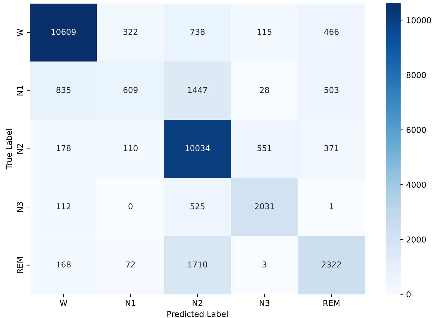
Confusion Matrix - ManualBiLSTM
