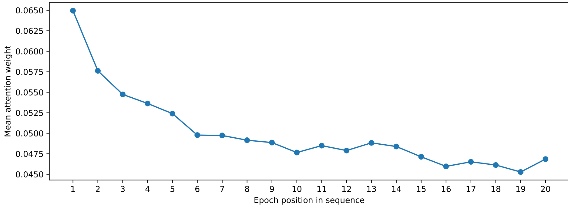
Mean Temporal Attention - FusionAttentionBiLSTM
