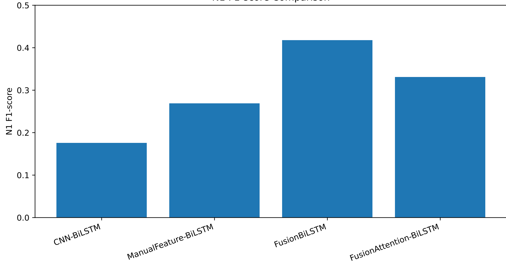
N1 F1-score Comparison
