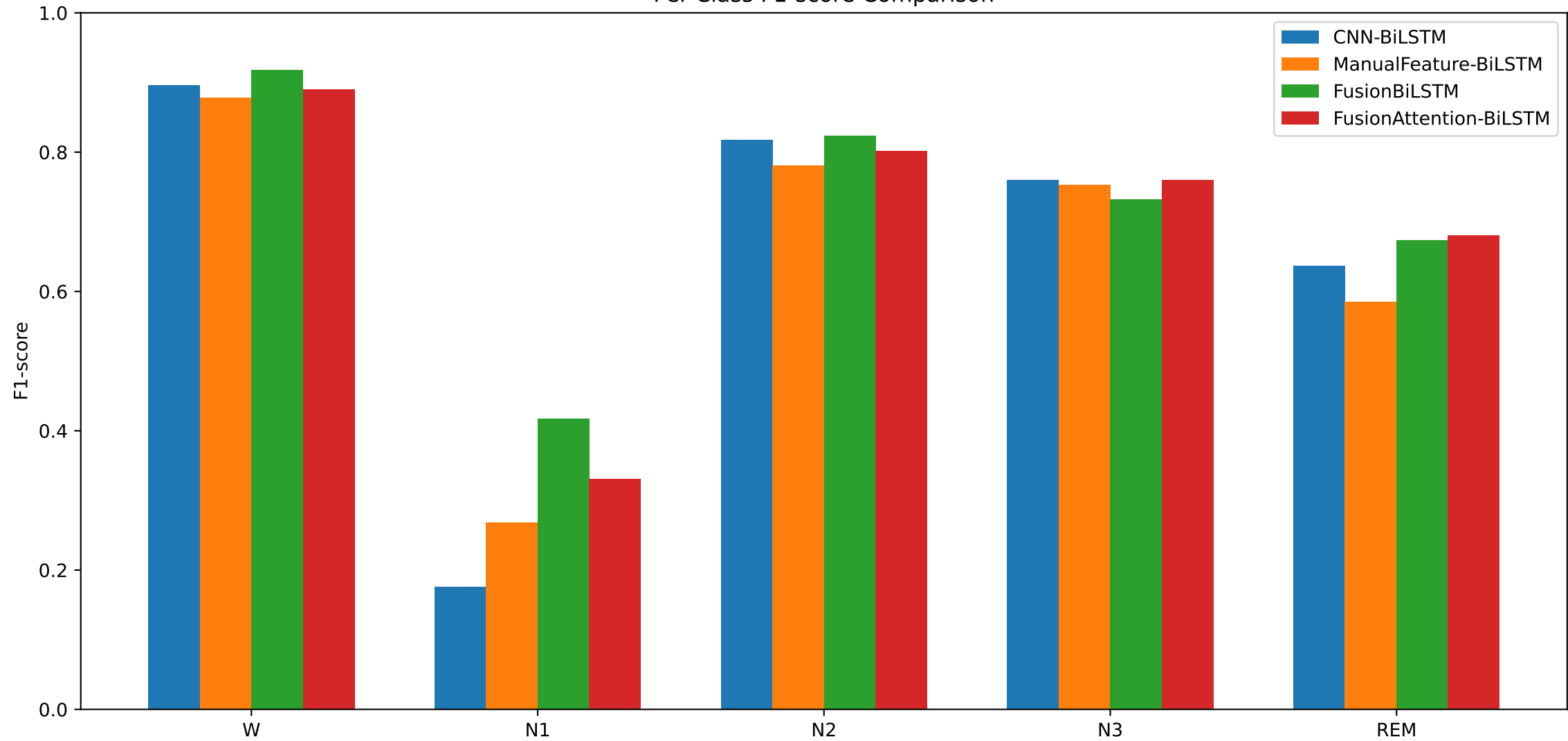
Per-Class F1-score Comparison
