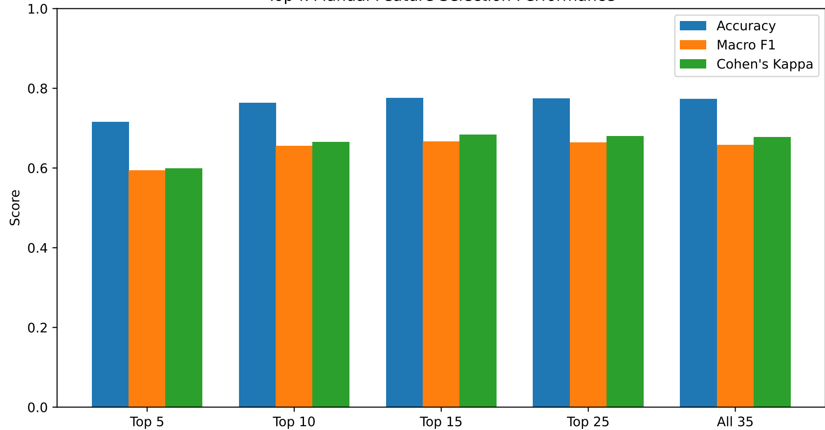
Top-k Manual Feature Selection Performance
