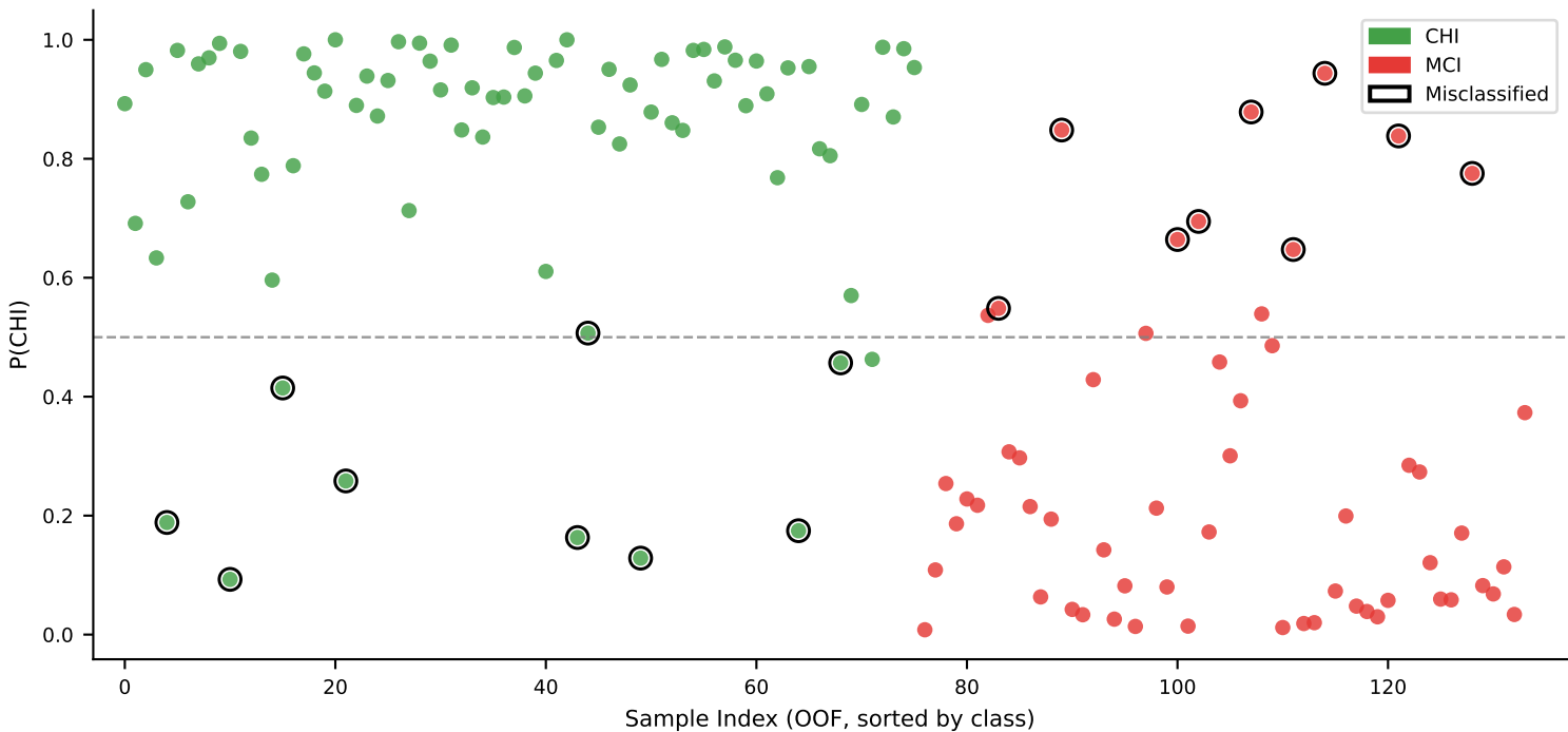
Classification Result - Acc 0.87 | Misclassified CHI 9/76 | Misclassified MCI 9/58
