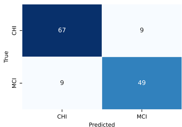
Confusion Matrix
