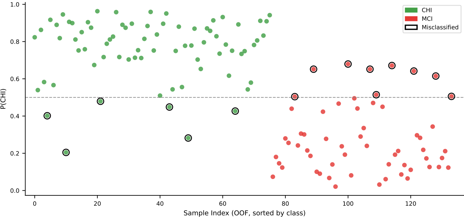
Classification Result - Acc 0.89 | Misclassified CHI 6/76 | Misclassified MCI 9/58
