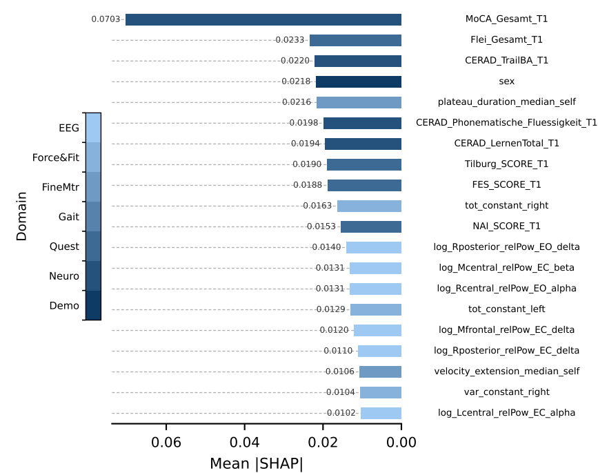
Top 20 - SHAP Importance
