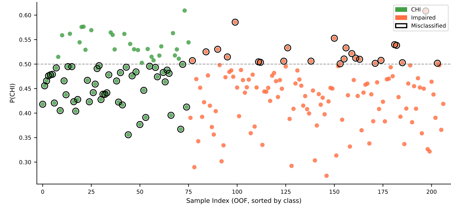
Classification Result - Acc 0.65 | Misclassified CHI 49/76 | Misclassified Impaired 24/131
