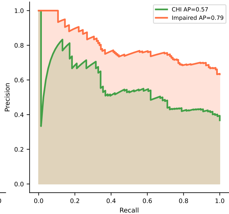
Precision-Recall
