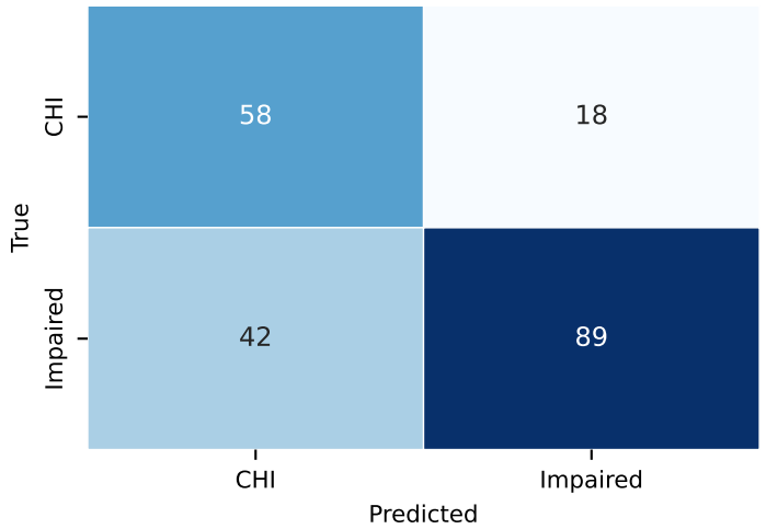
Confusion Matrix
