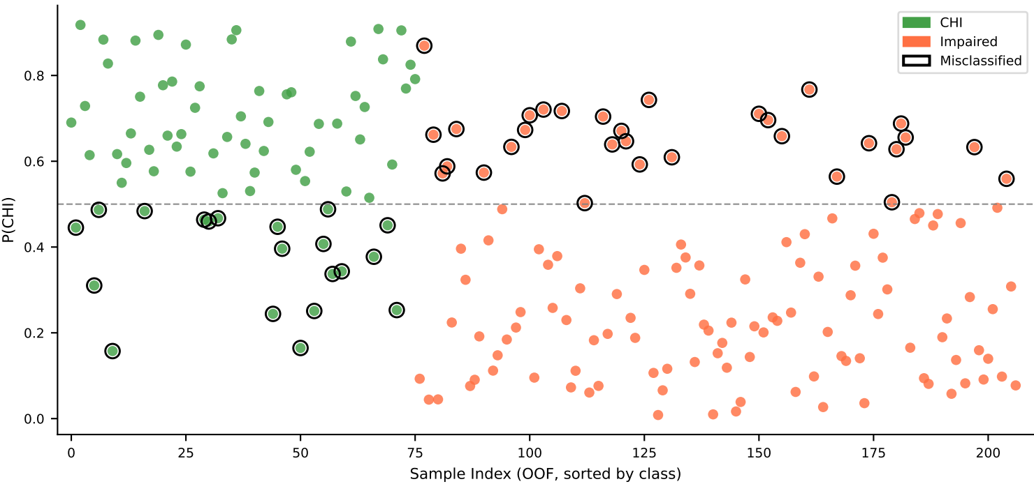
Classification Result - Acc 0.75 | Misclassified CHI 20/76 | Misclassified Impaired 31/131
