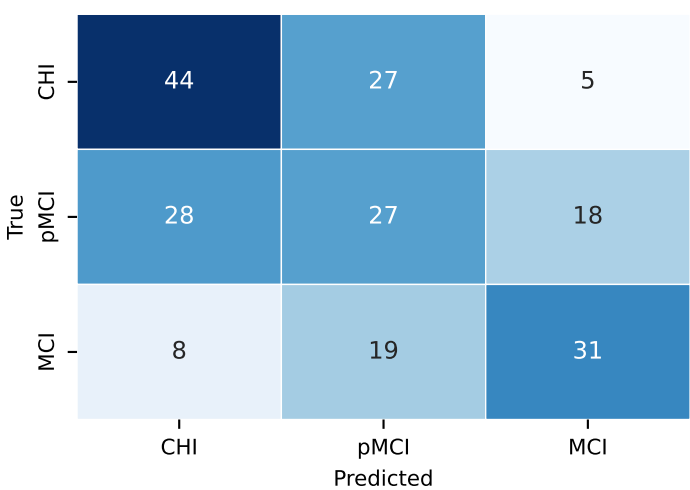
Confusion Matrix
