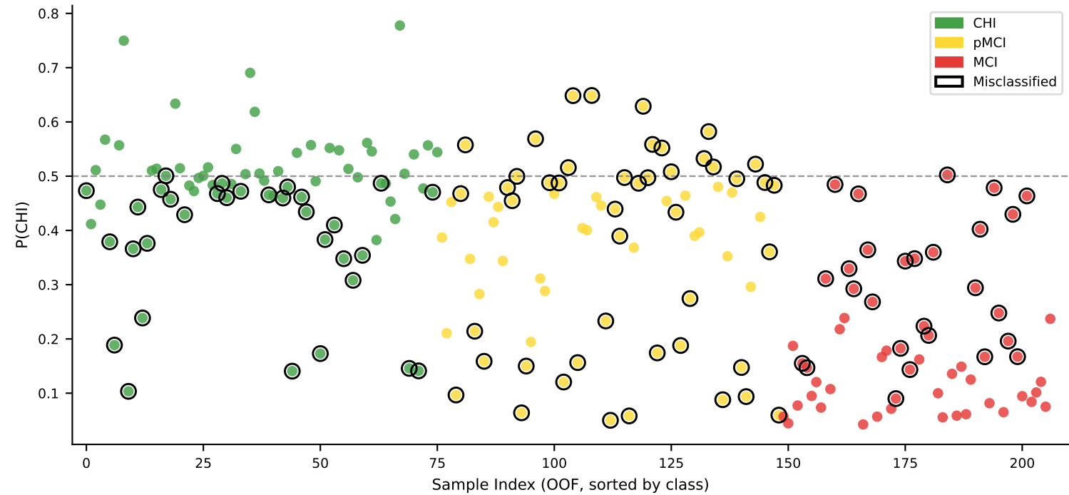
Classification Result - Acc 0.49 | Misclassified CHI 32/76 | Misclassified pMCI 46/73 | Misclassified MCI 27/58
