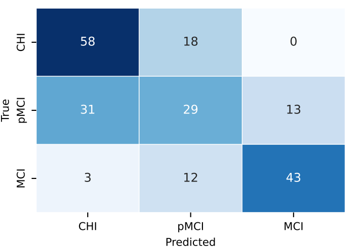
Confusion Matrix
