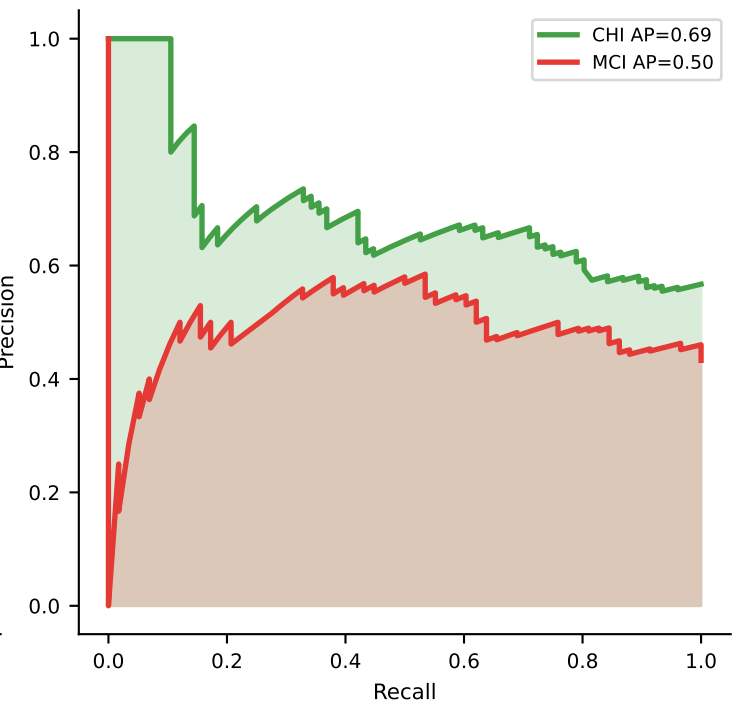
Precision-Recall
