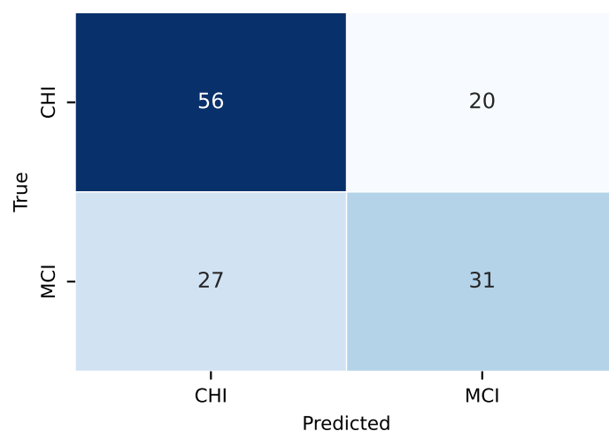
Confusion Matrix
