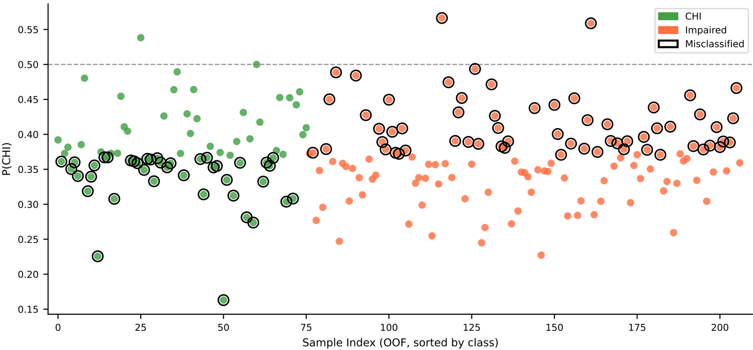
Classification Result - Acc 0.51 | Misclassified CHI 40/76 | Misclassified Impaired 61/131
