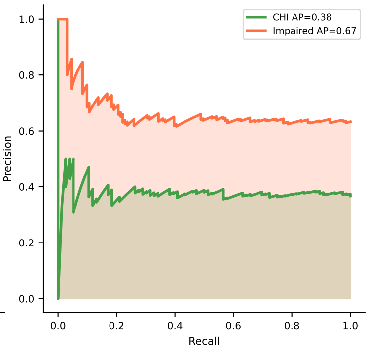
Precision-Recall
