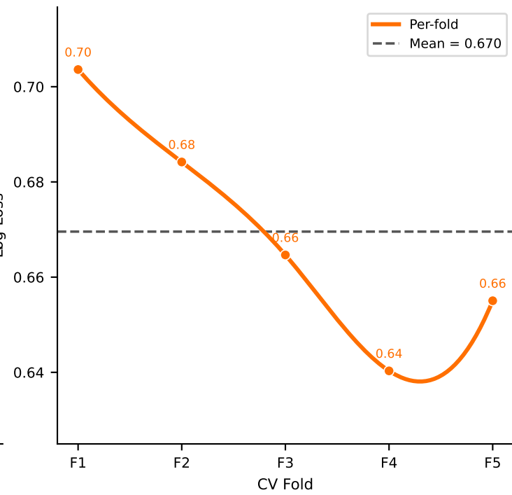
Log-Loss over 5 Folds
