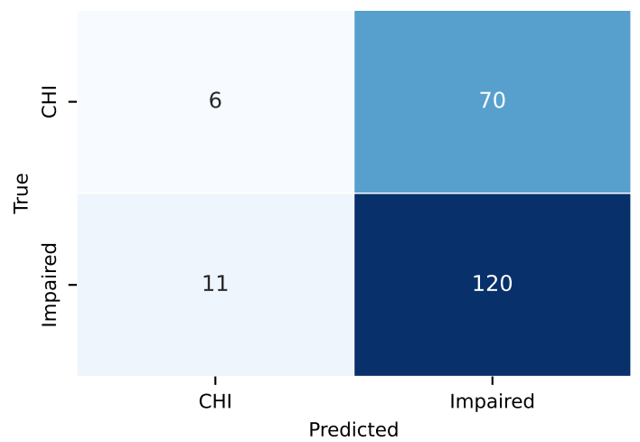
Confusion Matrix
