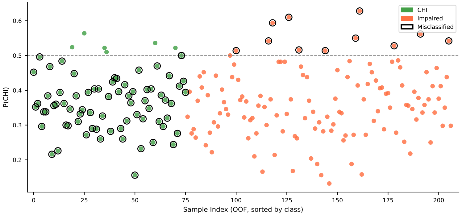
Classification Result - Acc 0.61 | Misclassified CHI 70/76 | Misclassified Impaired 11/131
