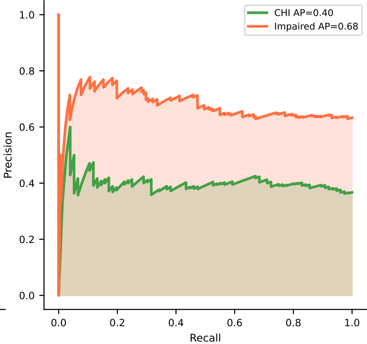
Precision-Recall
