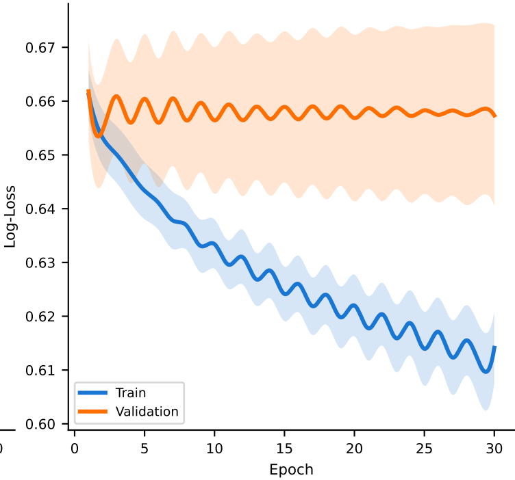
Loss over Epochs (mean±std, 5 folds)
