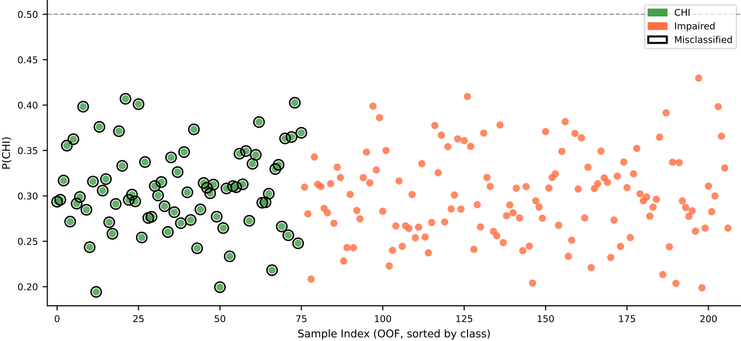
Classification Result - Acc 0.63 | Misclassified CHI 76/76 | Misclassified Impaired 0/131
