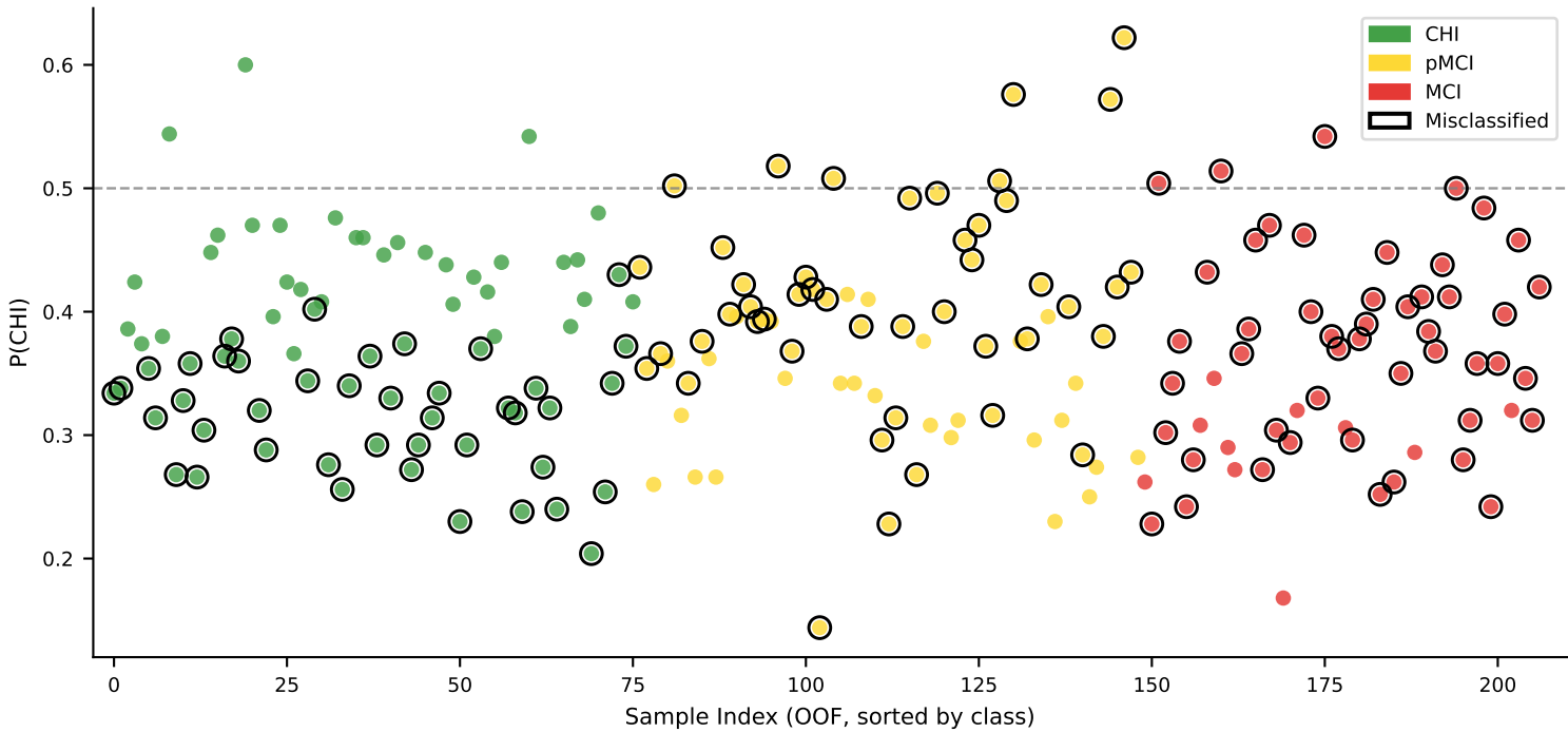
Classification Result - Acc 0.34 | Misclassified CHI 42/76 | Misclassified pMCI 46/73 | Misclassified MCI 48/58
