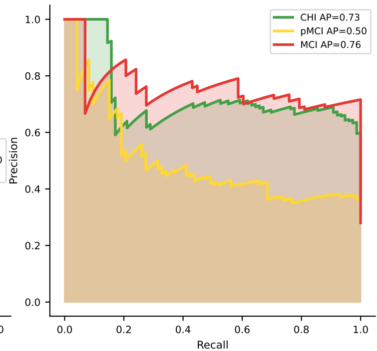
Precision-Recall
