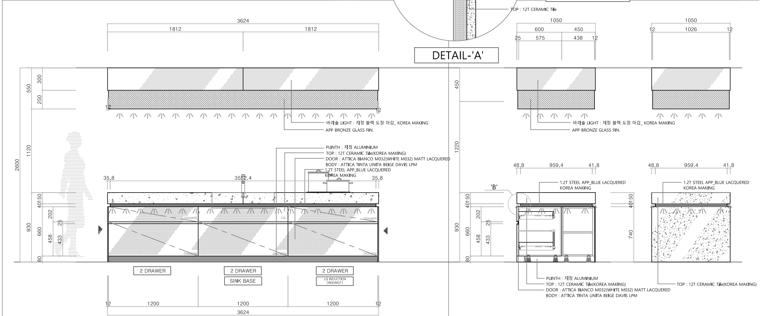
03 FRONT VIEW-'A'
