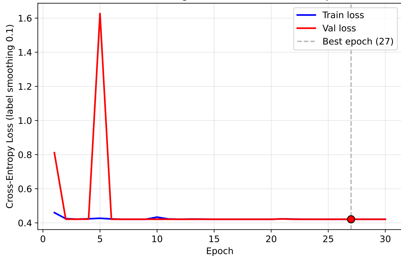
ResNet-18 Training Curve (seed 42, 30K samples)
