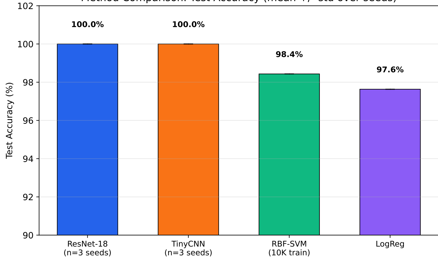
Method Comparison: Test Accuracy (mean +/- std over seeds)
