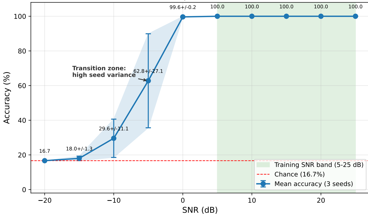
ResNet-18 HAR: Accuracy vs. SNR (3-seed mean \pm std)
