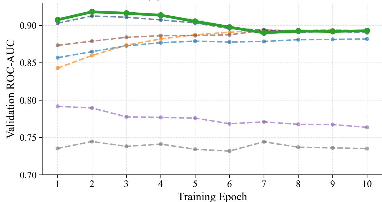
(b) Validation ROC-AUC
