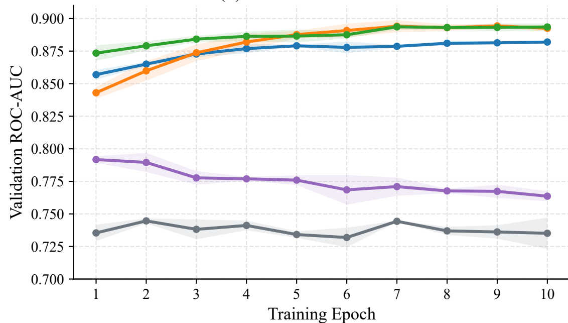
(b) Validation ROC-AUC
