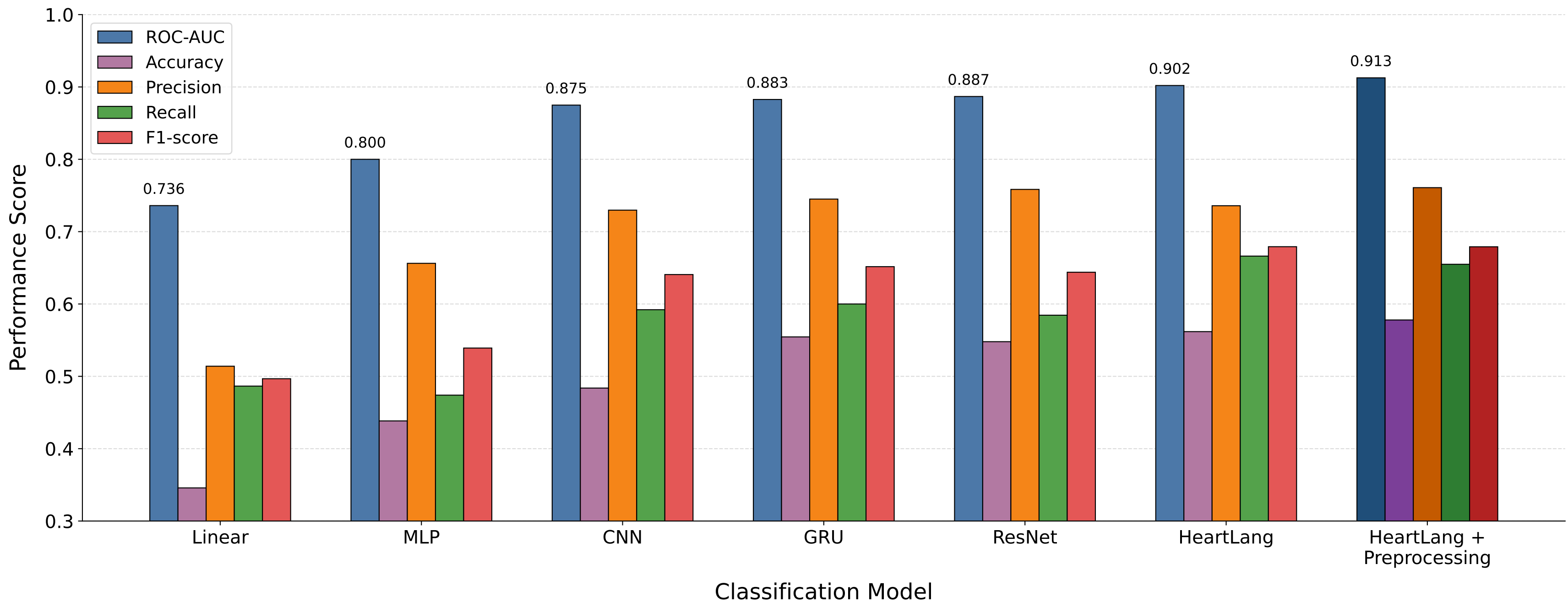
Performance Comparison of Baseline Models and Proposed HeartLang Framework
