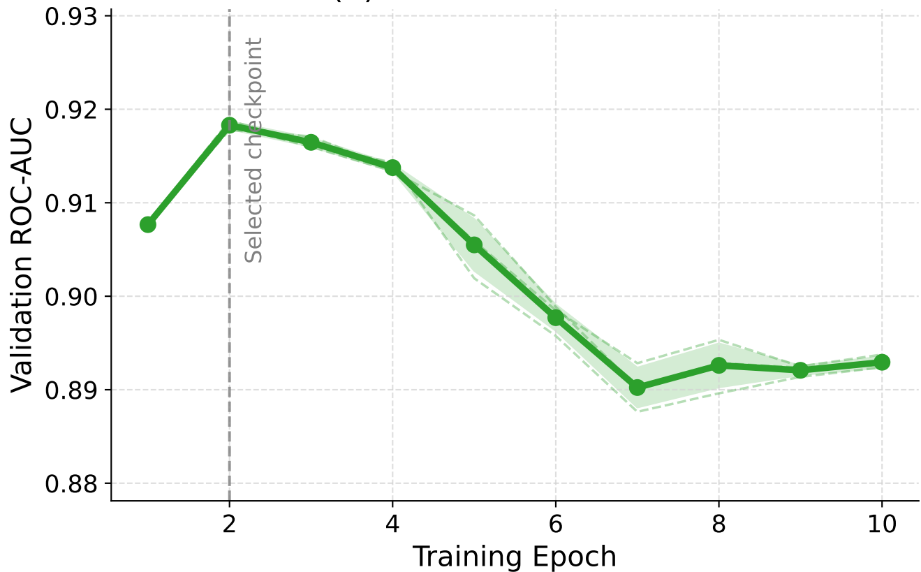
(b) Validation ROC-AUC
