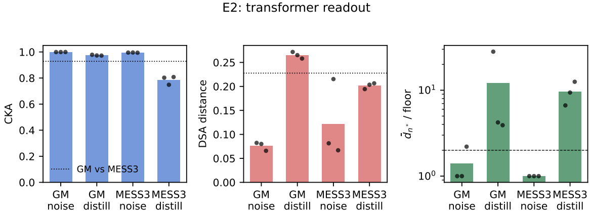
Figure 5: E2 summary: three metrics on transformer pairs (bars = mean over 3 seeds, points = seeds; dotted line = GM-vs-MESS3 cross anchor). \bar{d} shown at the amended plateau as a multiple of the same-process floor.
