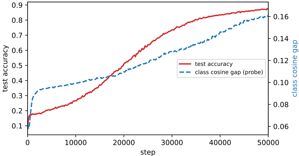
Structure forms early, behavior follows late (supcon-aug, seed 0)
