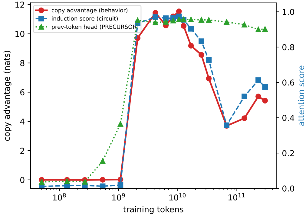
pythia-70m: precursor leads the capability cliff
