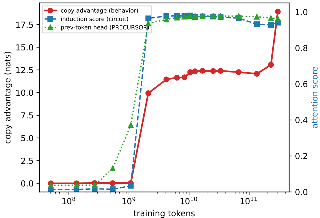
pythia-160m: precursor leads the capability cliff
