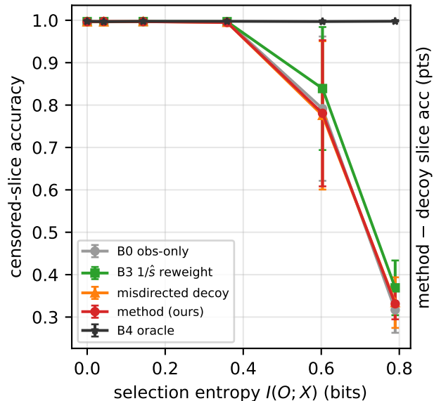
(a) slice accuracy
