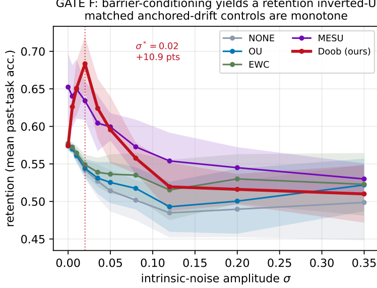
Figure 1: GATE F (Split-MNIST, 8 seeds, mean±sd) . The barrier-conditioned rule (Doob, red) rises from 57.4% at zero noise to 68.3% at an interior optimum \sigma^* = 0.02 (a 10.9-point lift; paired Wilcoxon p = 0.004 vs. zero, p = 0.004 vs. the high-noise end), then falls. The matched OU, EWC, MESU and naive anchors are monotone-decreasing in noise. Noise is a resource only when steered by the barrier.
