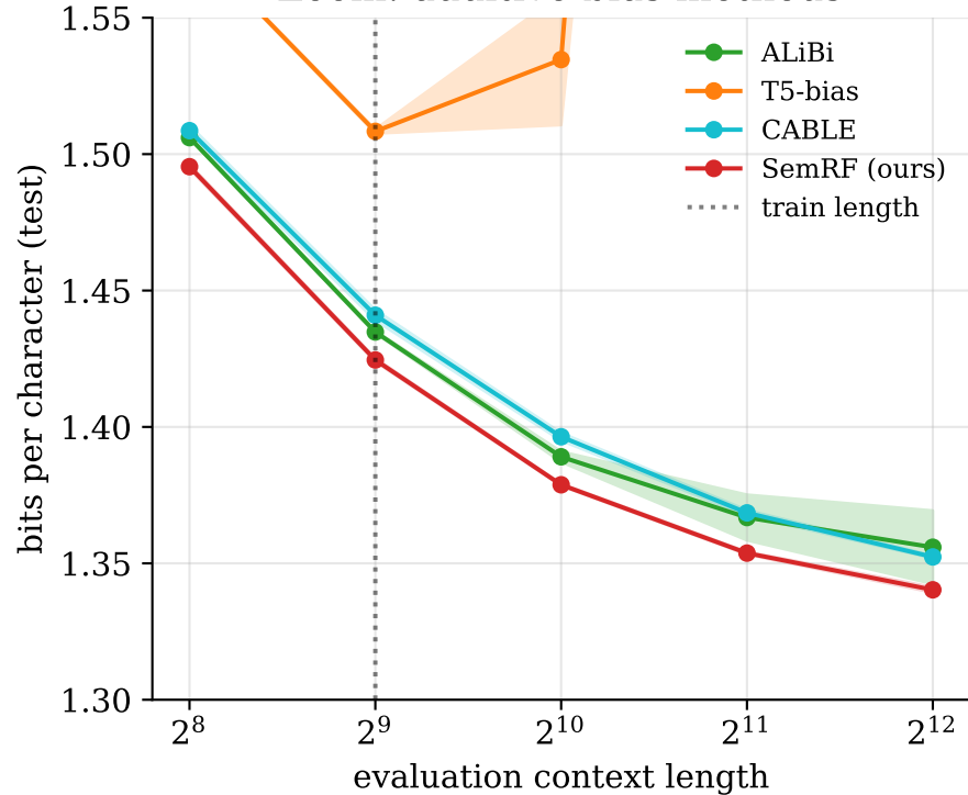
Zoom: additive-bias methods
