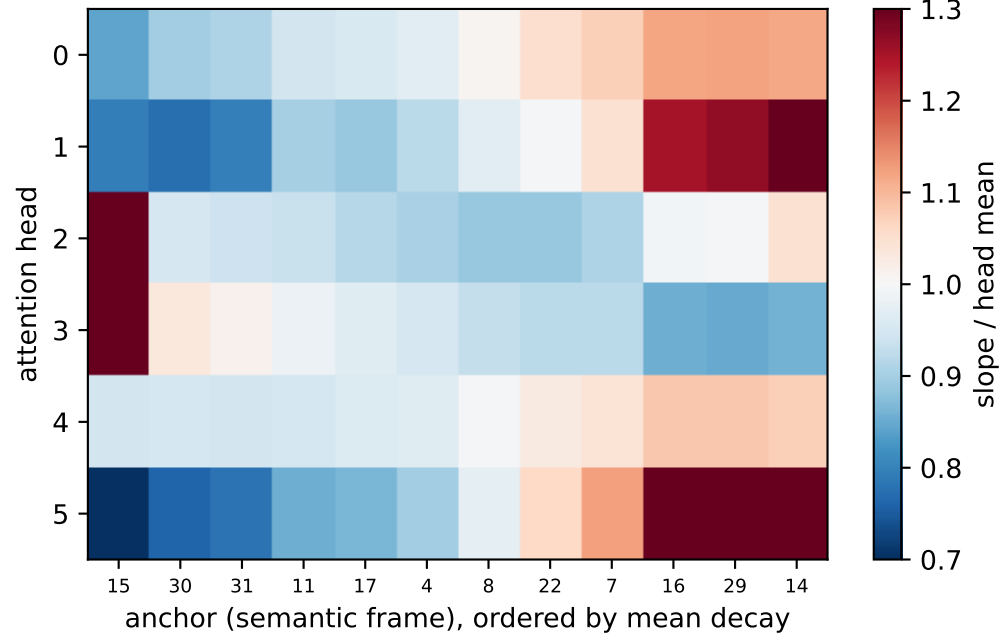
Relative to head mean (frame differentiation)
