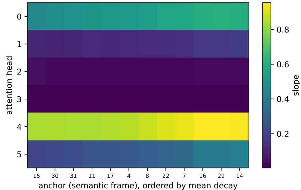
Decay slopes softplus( s_{hk} )
