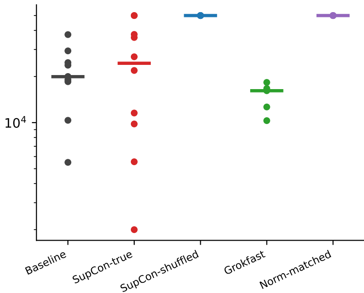
Epochs to generalization
